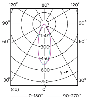
MASTER LEDspotMV 35W GU10 36D 260lm
